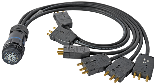
Break-In (6) male 20 Amp stage pins to female LSC19
